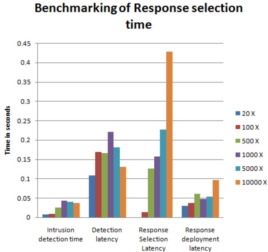
Figure 11. Benchmarking of response selection time
